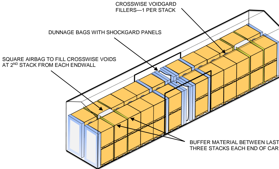
Figure 3 - Wood bins with Shock-Gard® filler panels and airbags in a 50 ft car
