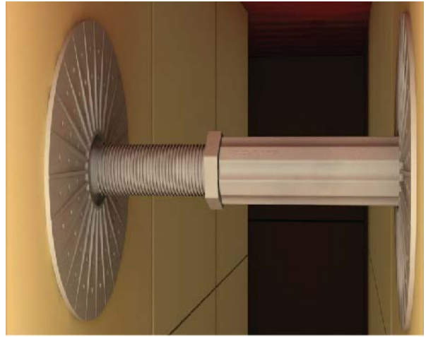
Figure 2 – Void-Gard® installed between bins in center void
