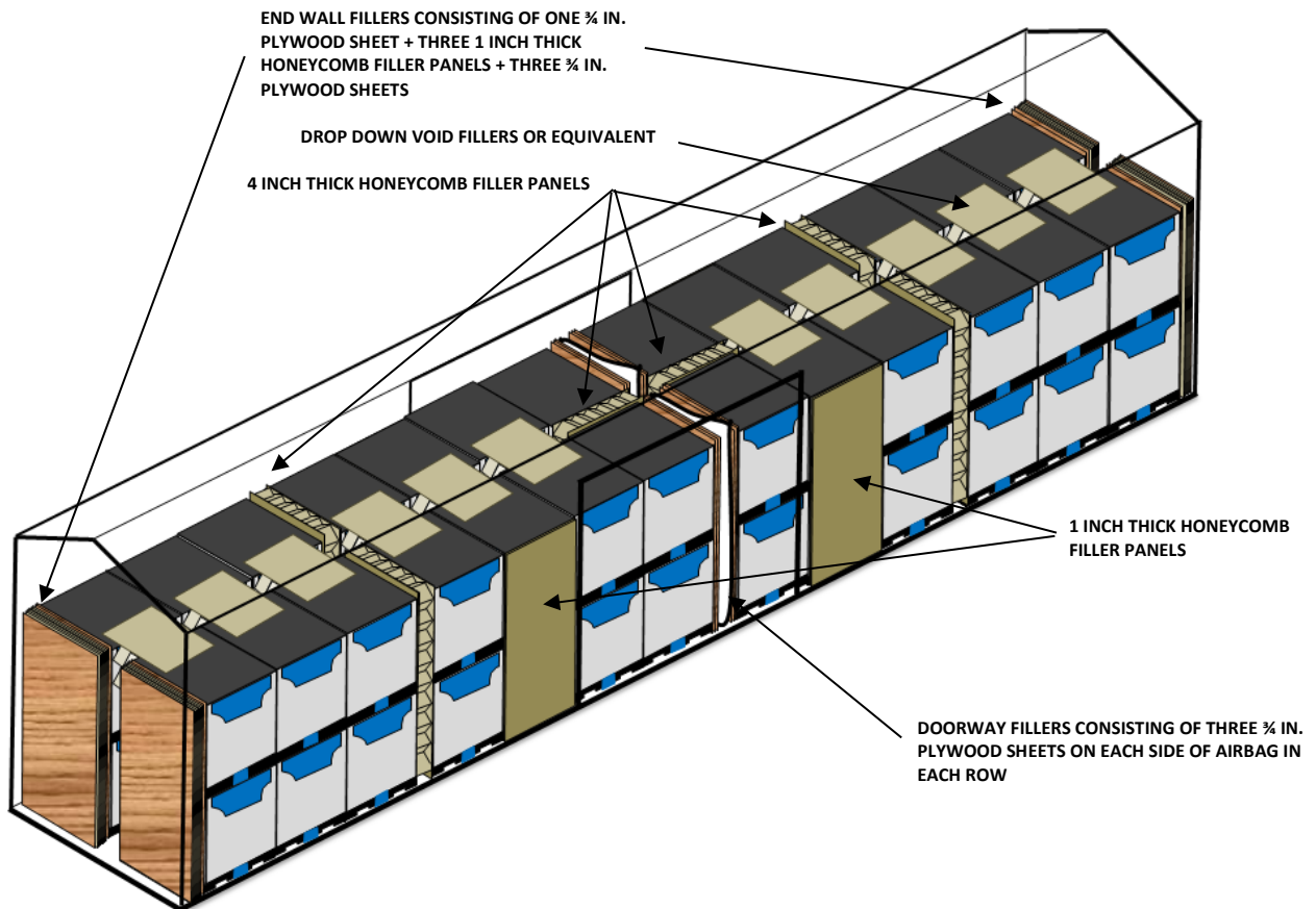
Figure 2 - Plastic intermediate bulk containers with dunnage bags
