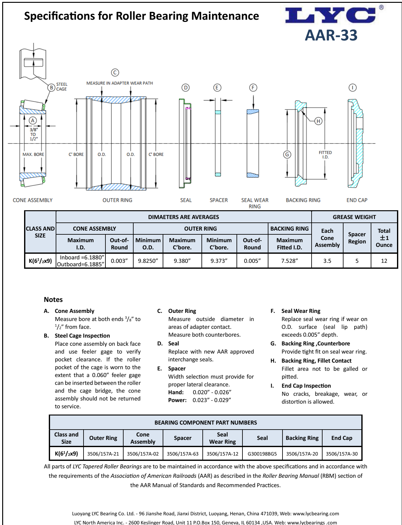
Fig. 3.7.28 LYC maintenance specifications AAR approval No. 33 Rule 3.7.2
