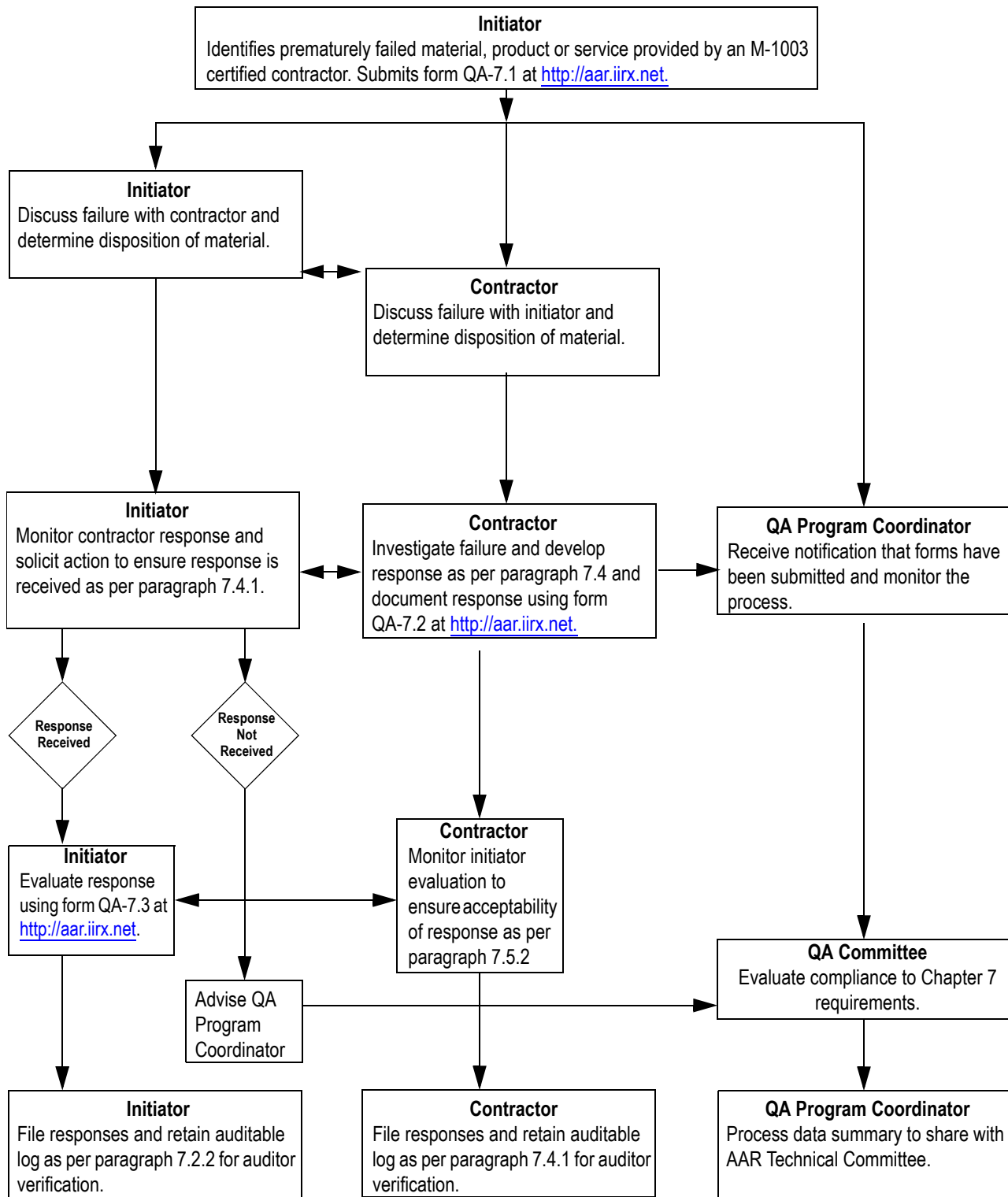
Fig. 7.1 Process map for nonconformance reporting
